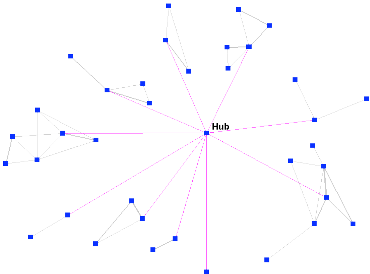
Figure 2 – Hub-and-Spoke Network
